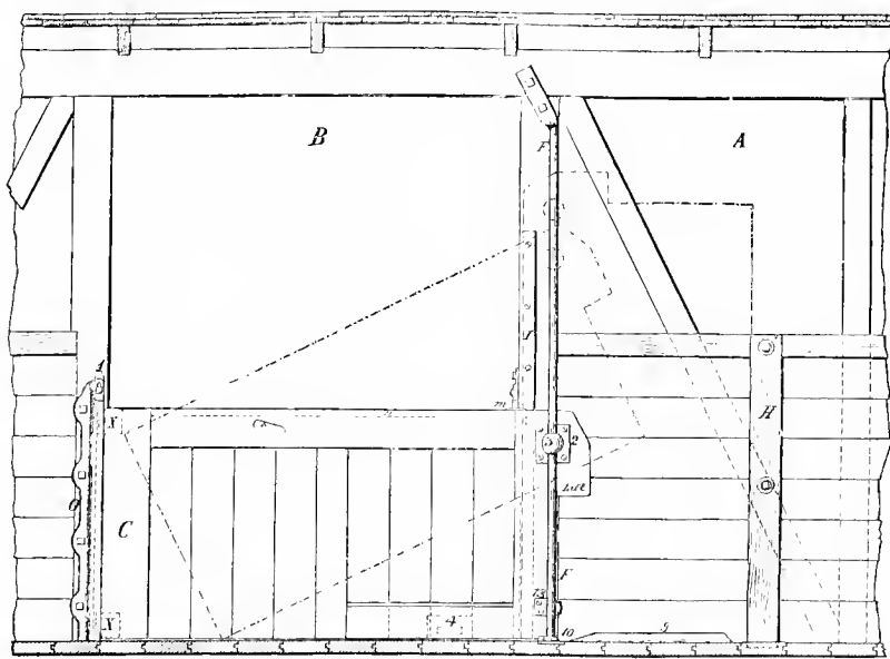
Fig. 1867. Interior Elevation.
